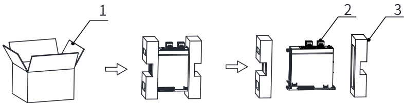
1. Carton; 2. Drive unit; 3. EPE
