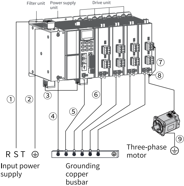
Figure 3-1 System grounding
