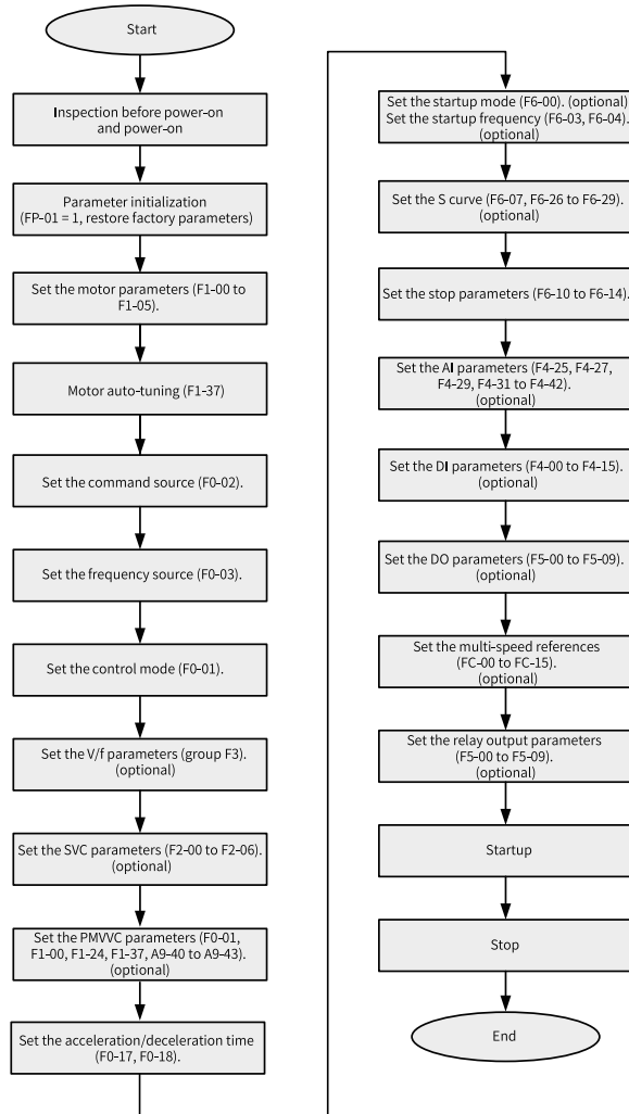
Figure 4-1 Basic commissioning flowchart
