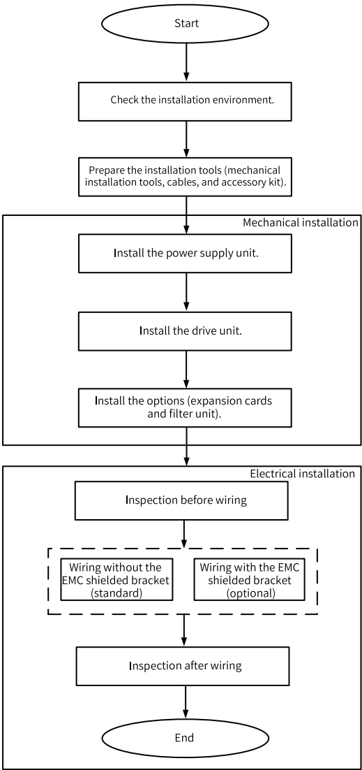
Figure 2-1 Installation flowchart
