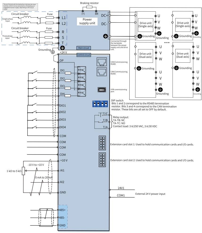
Figure -5 Electrical wiring
