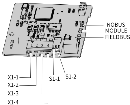
Figure 3-14 External connection of the MD580-SI-CAN1 module
