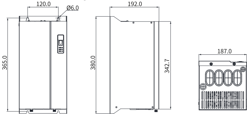
Figure 4-1 Outline dimensions of MDBUN-200-7T braking unit (unit: mm)
