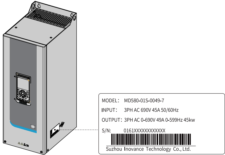
Figure 1-2 Nameplate description
