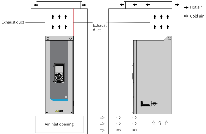
Figure 2-9 Using exhaust duct to prevent hot air recirculation
