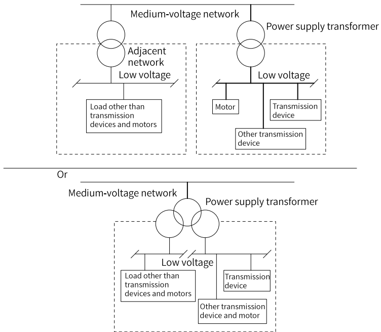
Figure 3-1 Selecting power supply transformers
