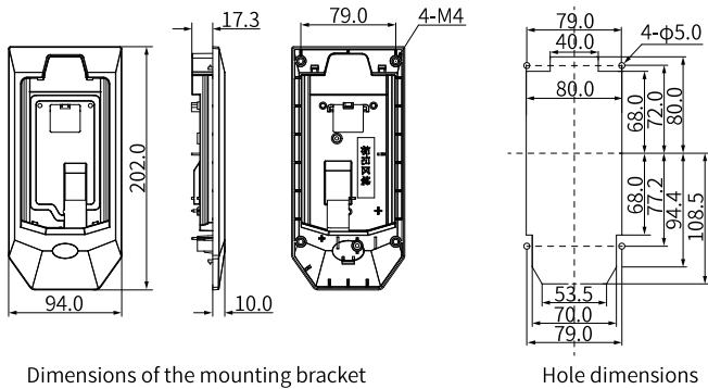
Figure 4-7 Bracket dimensions and hole sizes (mm) of the SOP-20-880
