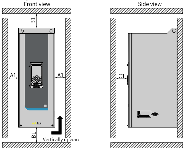
Figure 2-1 Clearance required for installing one AC drive
