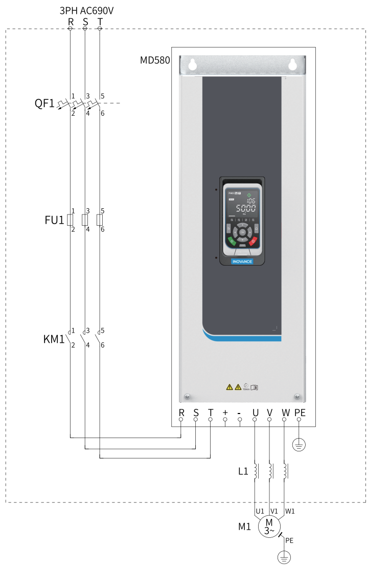
Figure 3-20 System composition
