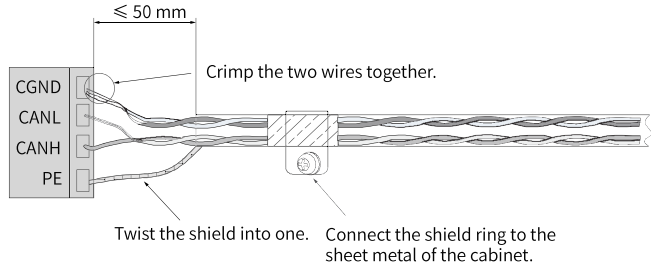
Figure 3-15 Terminal wiring
