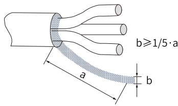
Figure 3-9 Lead wire of the motor cable shield
