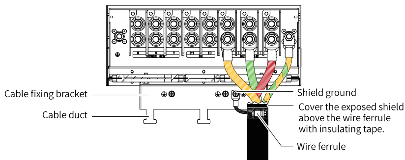
Figure 3-8 Shield wiring
