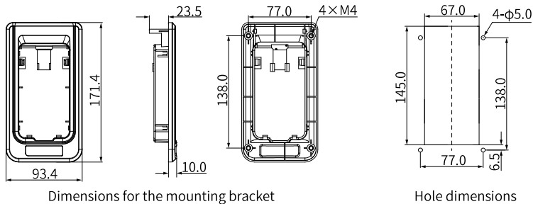
Figure 4-6 Bracket dimensions and hole sizes (mm) of the MDKE-10
