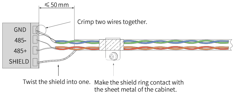
Figure 3-17 Terminal wiring
