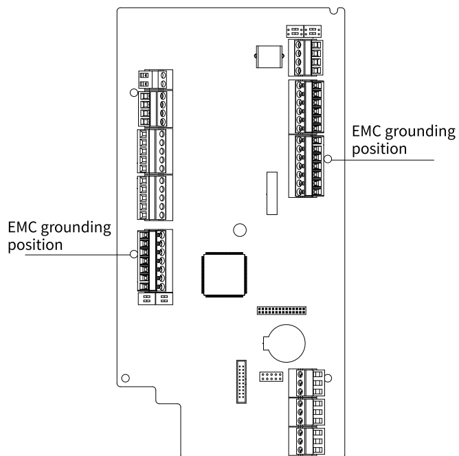
Figure 3-43 Control board grounding
