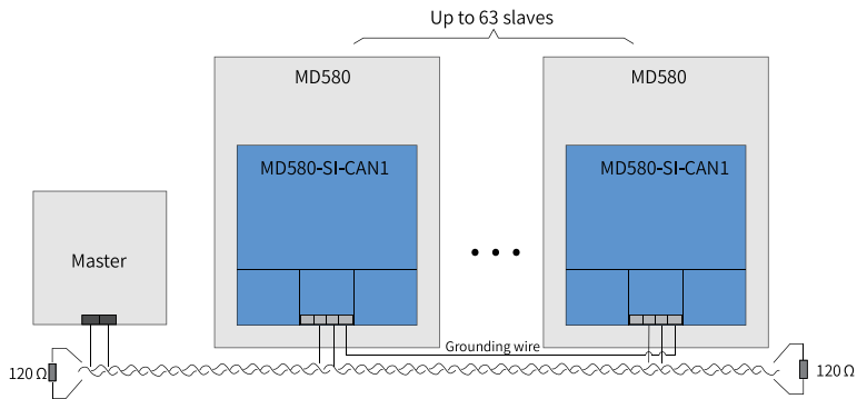
Figure 3-27 Networking diagram
