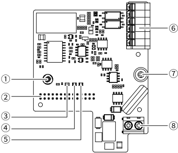
Figure 4-50 Components
