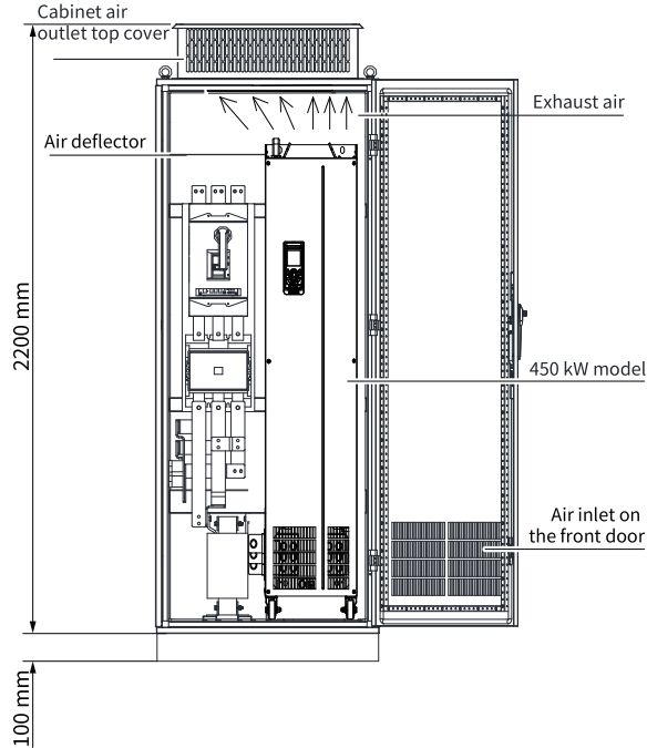
Figure 2-9 Self-ventilated cabinet
