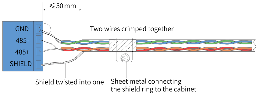
Figure 3-29 Terminal wiring
