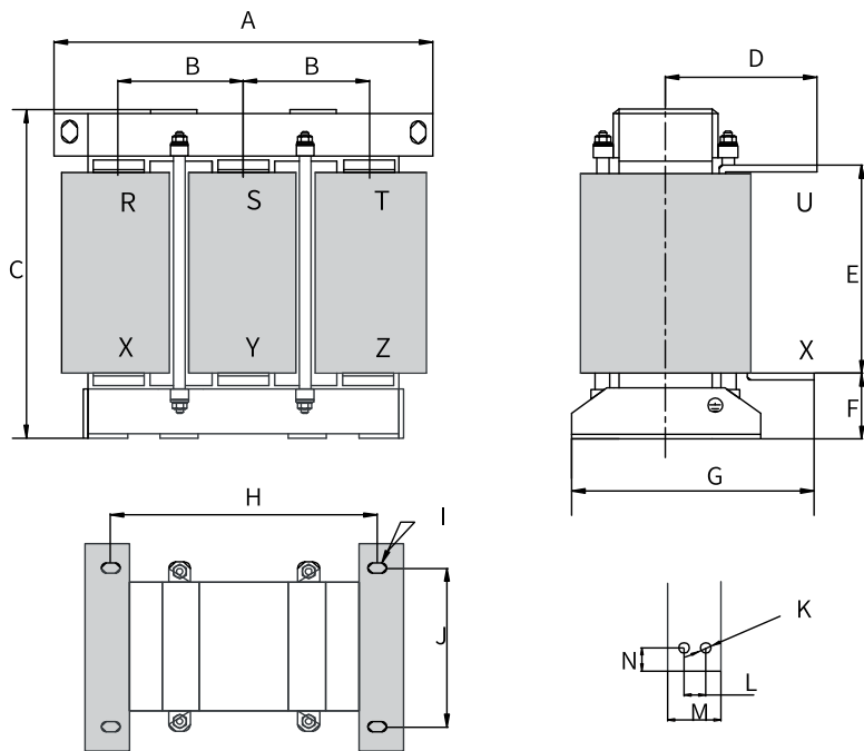
Figure 4-20 Dimensions of AC input reactors (800-1000 A)
