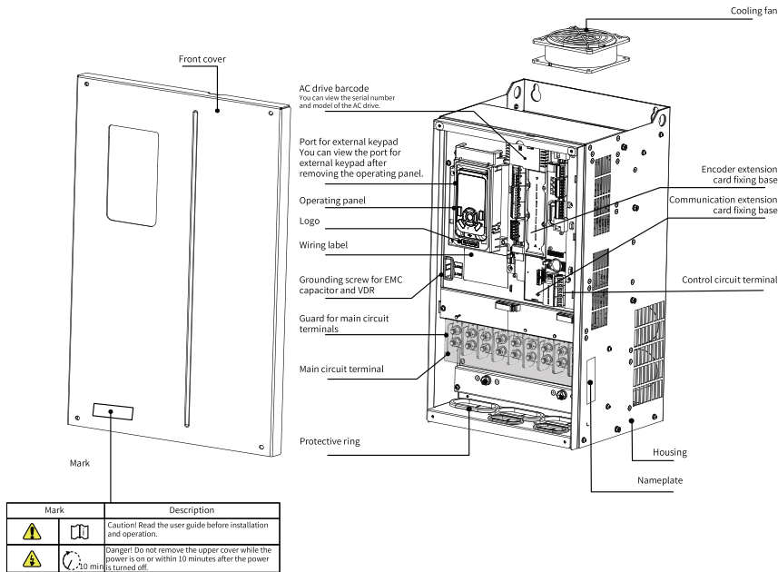
Figure 1-4 Components of T7 to T9 models
