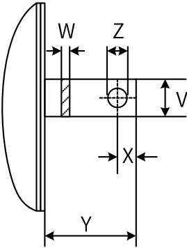
Figure 4-24 Dimensions of copper busbars
