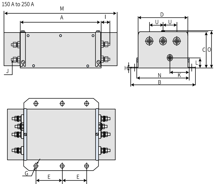
Figure 4-22 Dimensions of FN 3359 series filters (150-250 A)
