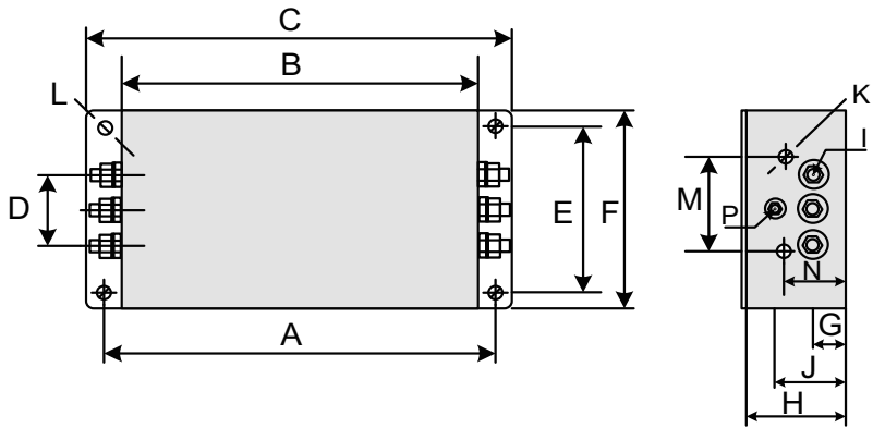
Figure 4-25 Dimensions of Jianli filters (50-200 A)
