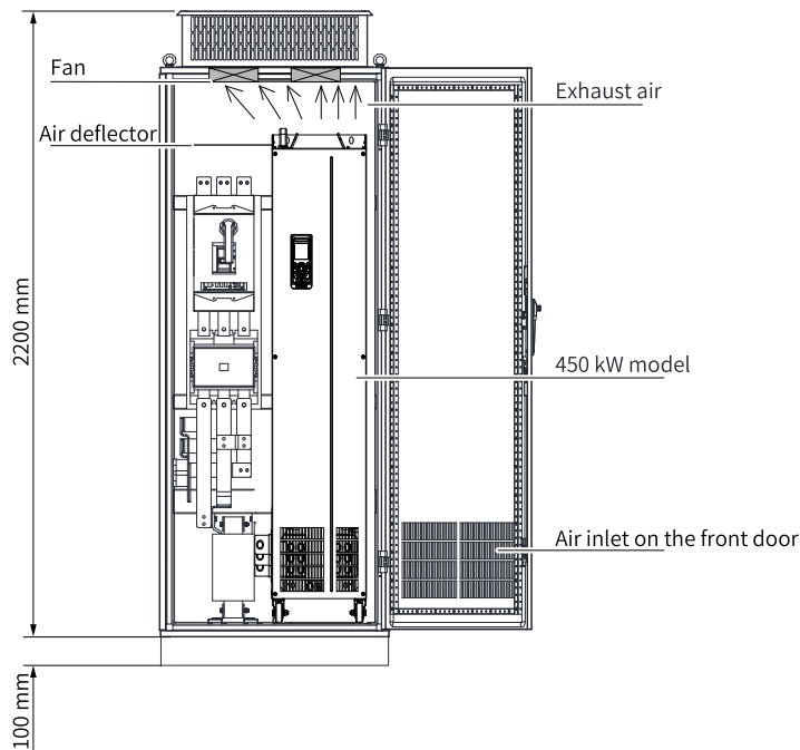
Figure 2-10 Forced-ventilated cabinet (with fans at the top of the cabinet)
