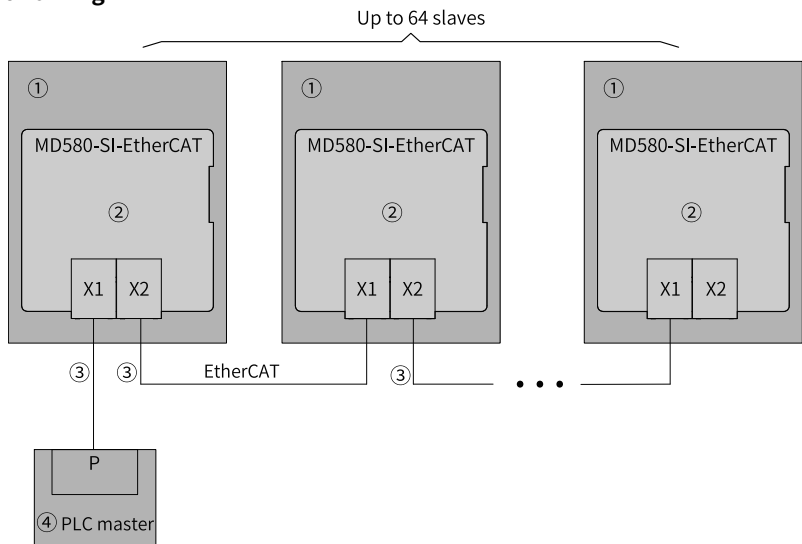
Figure 3-41 Chain networking topology
