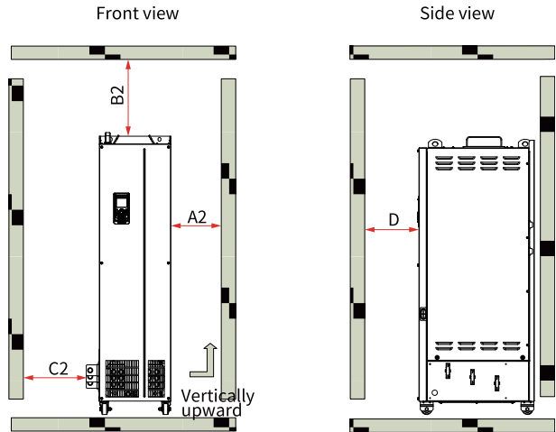
Figure 2-8 Installation clearance (T10 to T12 models)
