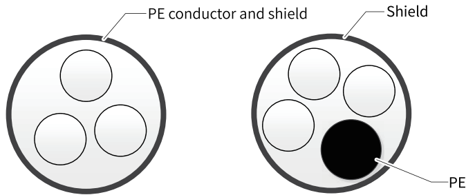
Figure 3-9 Recommended power cable types
