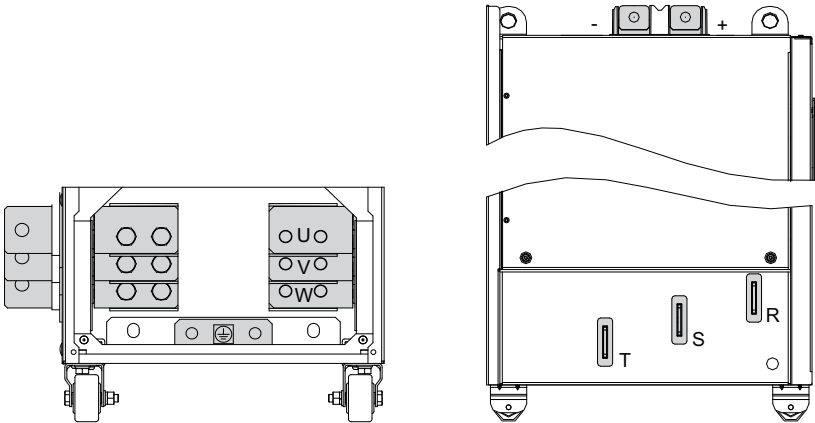
Figure 3-7 Layout of main circuit terminals for T10 to T12 models
