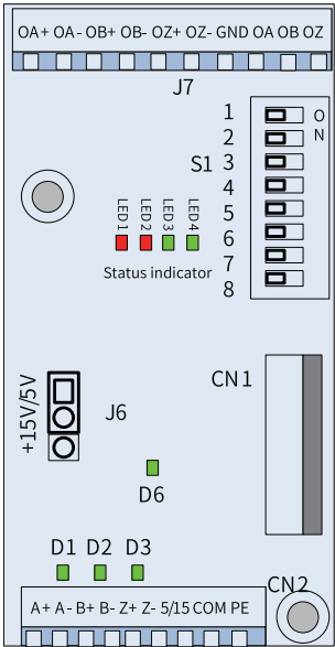
Figure 4-52 Layout of MD38PGMD terminals
