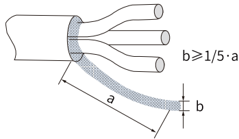
Figure 3-13 Drain wire of the motor cable shield
