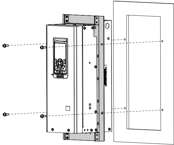
Figure 2-17 Through-hole mounting (T1 to T9 models)
