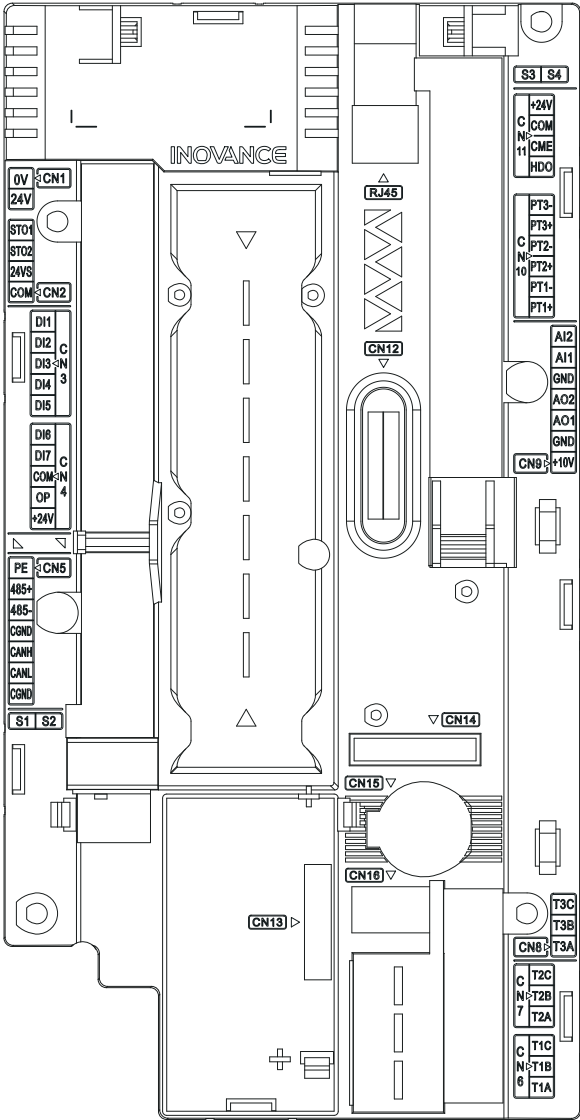
Figure 3-14 Layout of control circuit terminals
