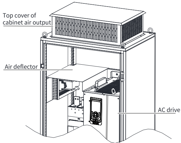
Figure 2-11 Insulation barrier in the cabinet
