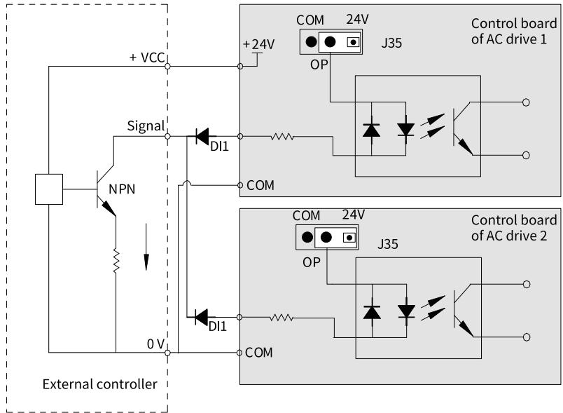
Figure 3-18 Parallel connection of DI of multiple AC drives in the sink mode
