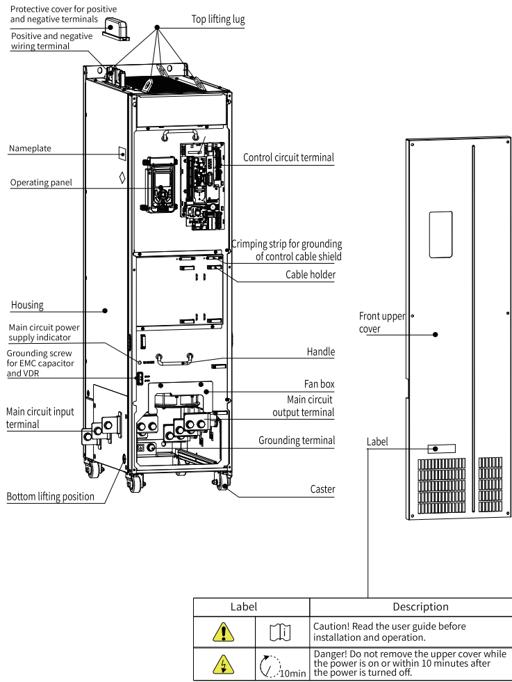
Figure 1-5 Components of T10 to T12 models (without an AC output reactor)
