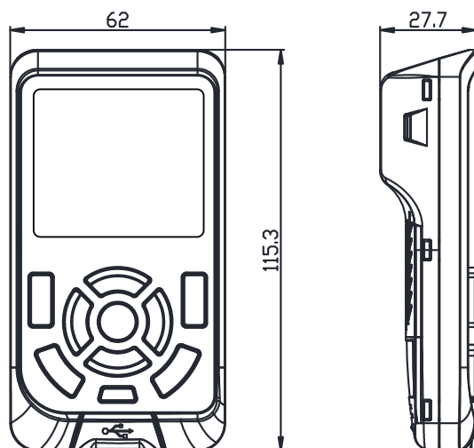
Figure 4-47 Dimensions of MDKE-10 LED (unit: mm)
