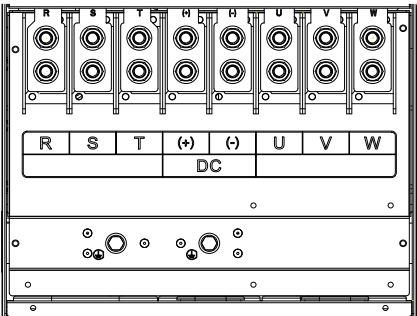
Figure 3-6 Layout of main circuit terminals for T9 models
