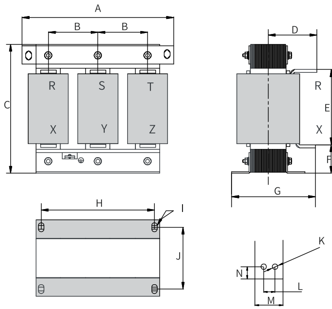
Figure 4-19 Dimensions of AC input reactors (490 A/660 A)
