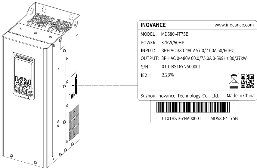
Figure 1-2 Nameplate and naming rules
