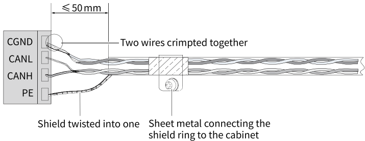
Figure 3-26 Terminal wiring
