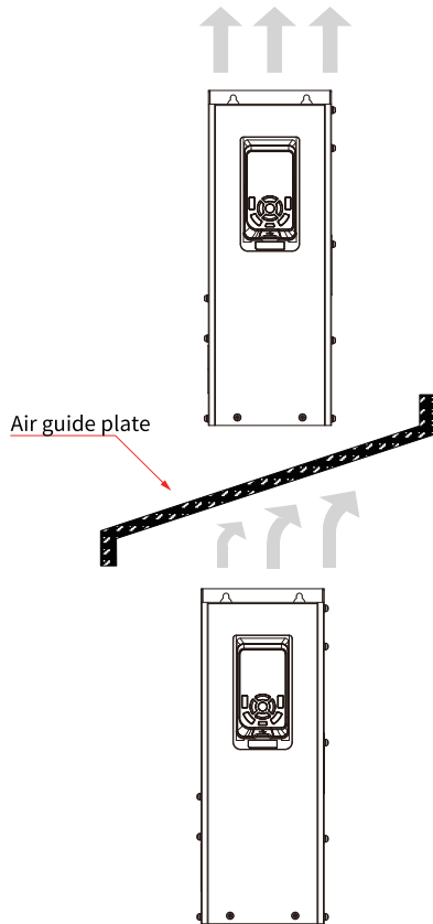
Figure 2-7 Installing one above another (T1 to T9 models)
