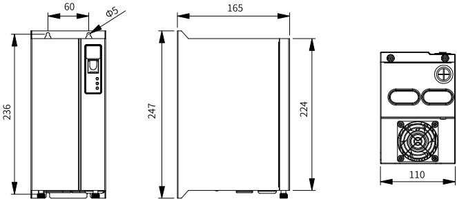
Figure 4-30 Dimensions of MDBUN series braking units (MDBUN-45-2T to MDBUN-90-2T; MDBUN-45-T to MDBUN-90-T; MDBUN-45-5T to MDBUN-90-5T) (mm)
