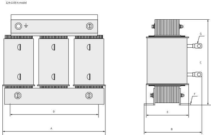
Figure 4-44 Dimensions of output reactors (124–1100 A)
