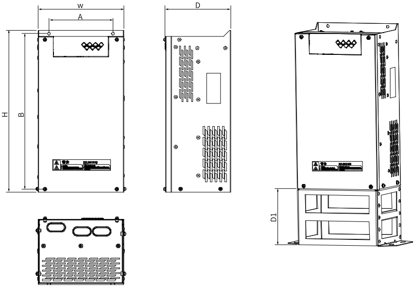
Figure 4-32 Dimensions of MD051 series AFE unit (unit: mm)
