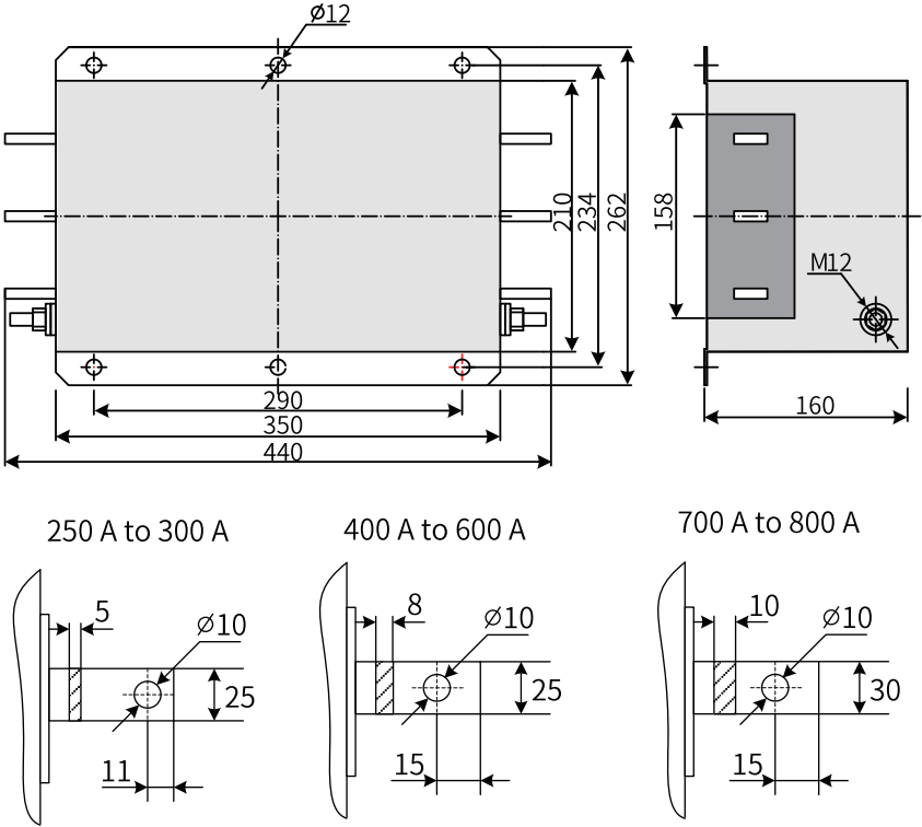
Figure 4-26 Dimensions of Jianli filters (250-800 A, unit: mm)
