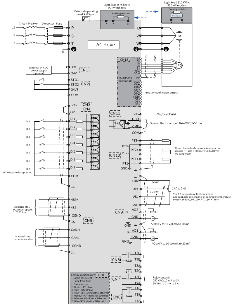
Figure 3-2 Standard wiring
