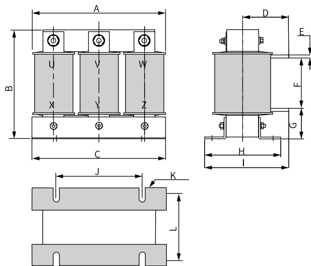
Figure 4-39 Dimensions of AC output reactors (80-120 A)
