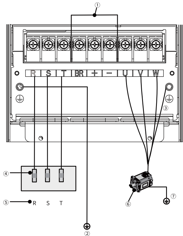
Figure 3-44 Main circuit grounding
