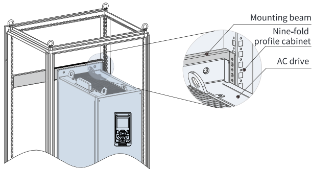
Figure 2-20 3D of a cabinet for T10 and T12 models
