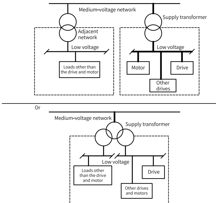
Figure 3-3 Selecting a supply transformer
