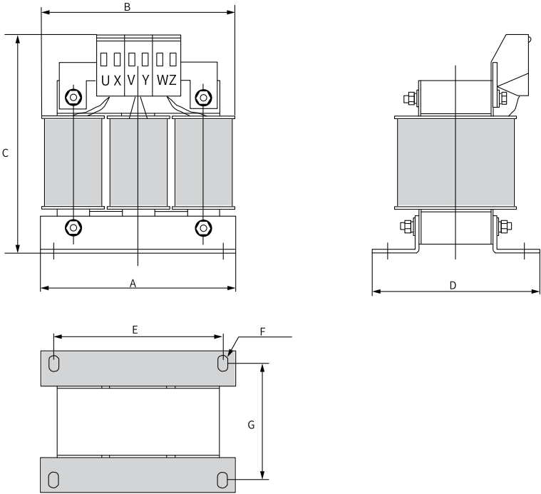
Figure 4-35 Dimensions of AC output reactors (5-10 A)
