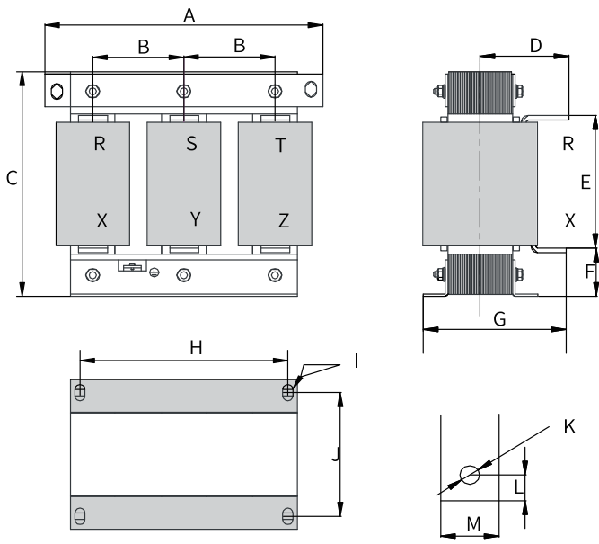
Figure 4-18 Dimensions of AC input reactors (150-330 A)
