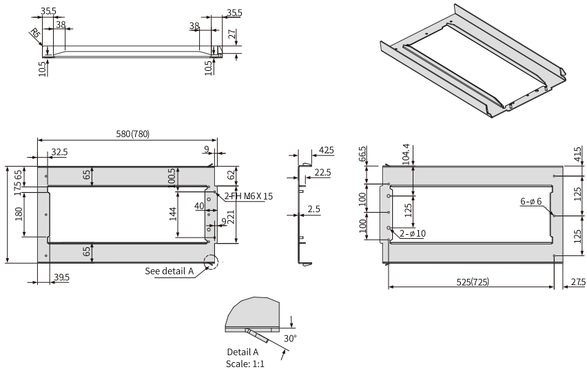
Figure 4-3 Dimensions of bottom mounting bracket for T12 models
