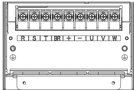
Figure 3-4 Layout of main circuit terminals for T1 to T4 models
