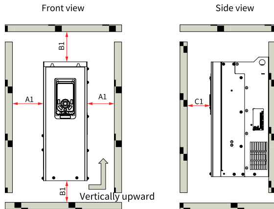
Figure 2-5 Clearance for installing one AC drive (T1 to T9 models)
