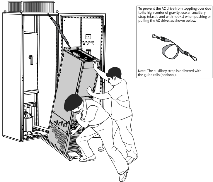
Figure 2-25 Pushing the AC drive into the cabinet
