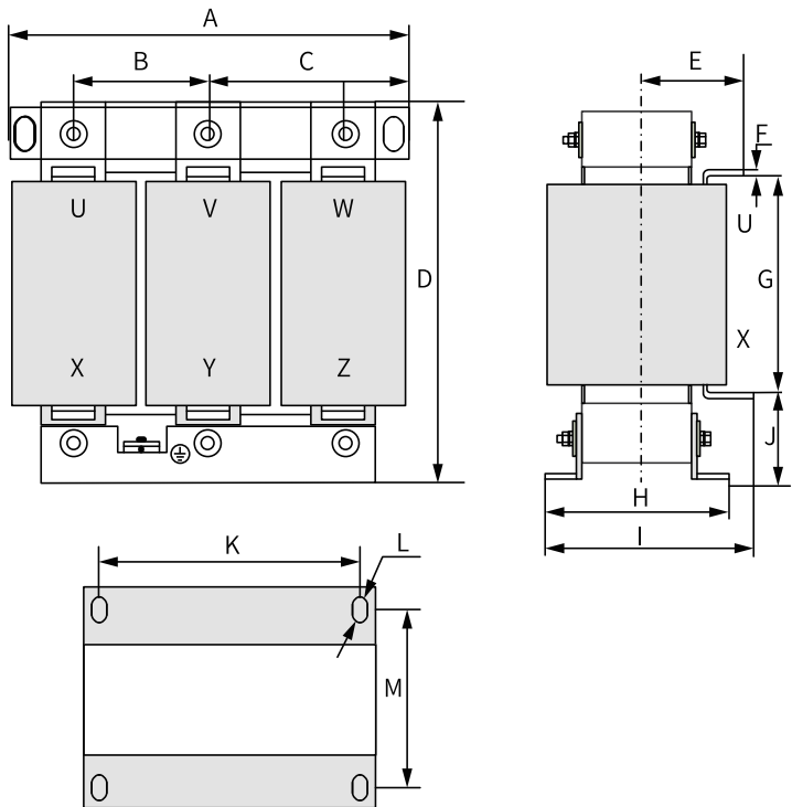
Figure 4-40 Dimensions of AC output reactors (150-250 A)
