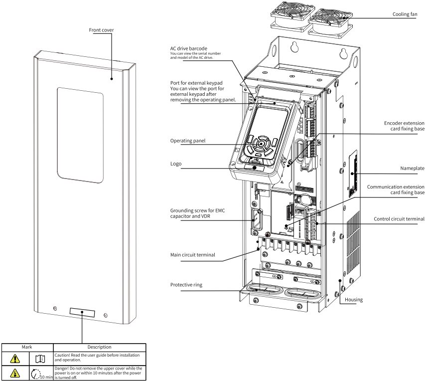
Figure 1-3 Components of T1 to T6 models
