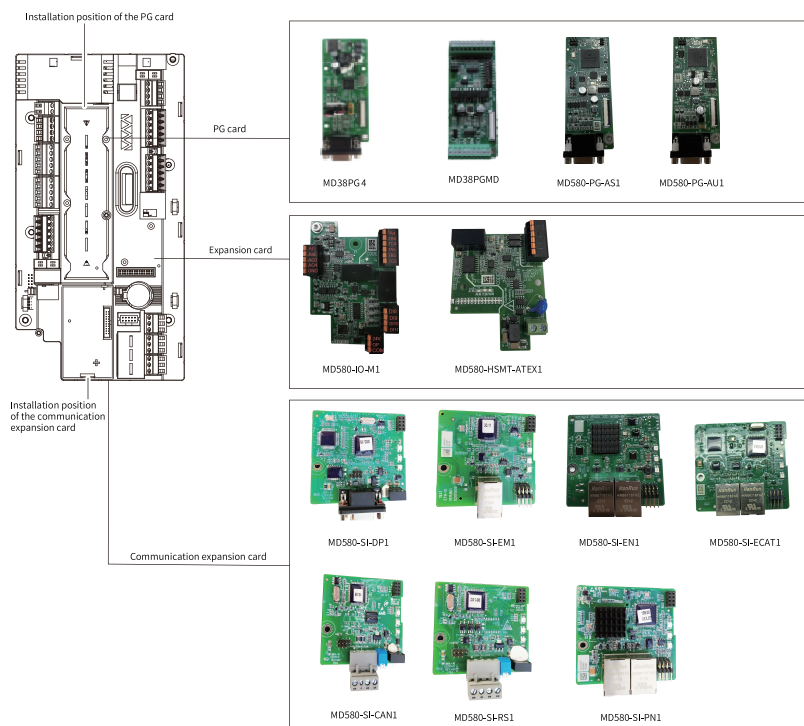
Figure 4-49 Installation positions of expansion cards
