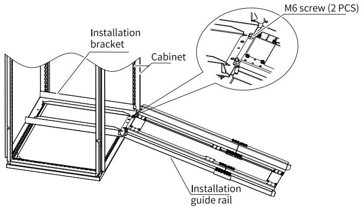
Figure 2-23 Mounting the guide rails on the cabinet
