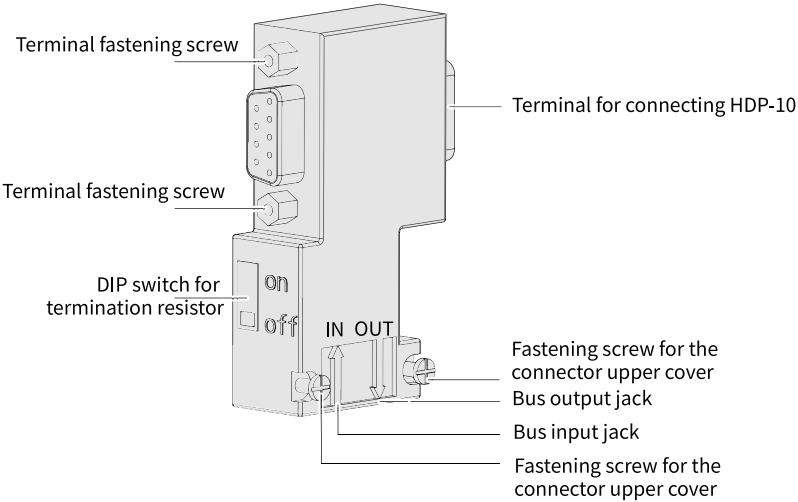
Figure 3-31 Bus connector
