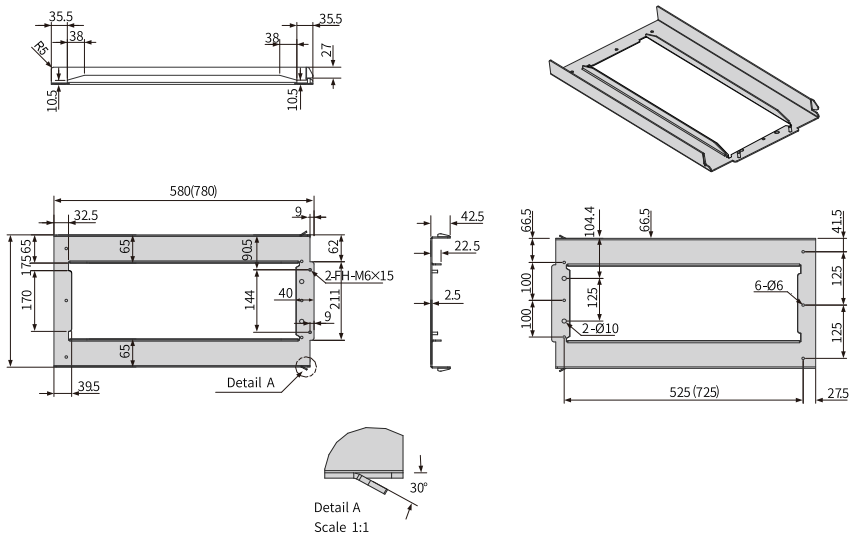
Figure 4-2 Dimensions of bottom mounting bracket for T11 models
