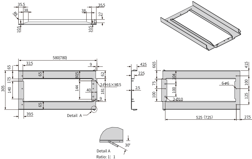
Figure 4-1 Dimensions of bottom mounting bracket for T10 models
