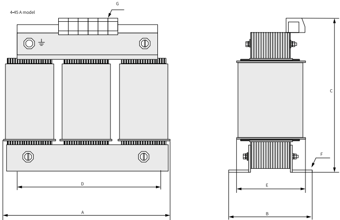
Figure 4-42 Dimensions of output reactors (4–45 A)
