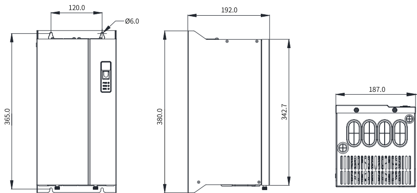
Figure 4-31 Dimensions of MDBUN series braking units (MDBUN-200-T, MDBUN-200-5T, MDBUN-200-7T) (mm)
