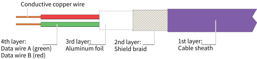
Figure 3-30 Internal layer of the bus
