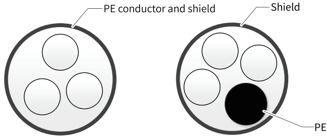
Figure 3-8 Recommended power cable types
