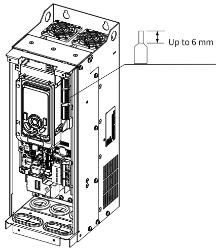
Figure 3-23 Requirements on tubular terminals of the control circuit cable
