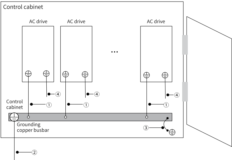
Figure 3-45 Grounding multiple AC drives installed side by side
