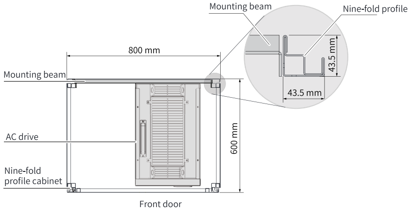
Figure 2-19 Top view of a cabinet for T10 and T12 models
