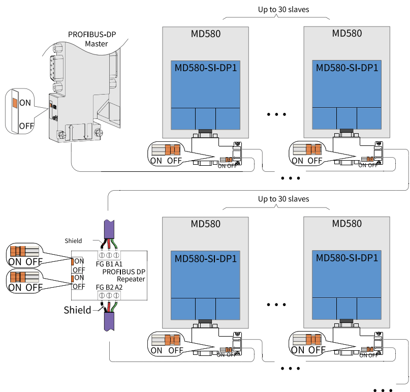
Figure 3-34 Multi-drive system connection with repeaters
