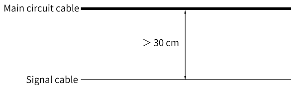
Figure 3-10 Cable routing
