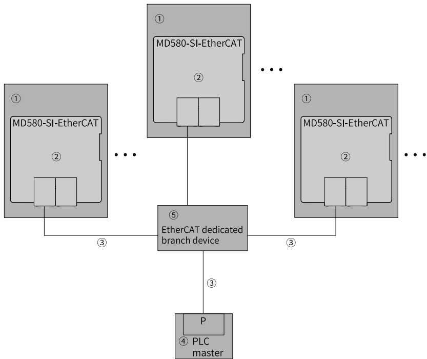
Figure 3-42 Chain networking topology
