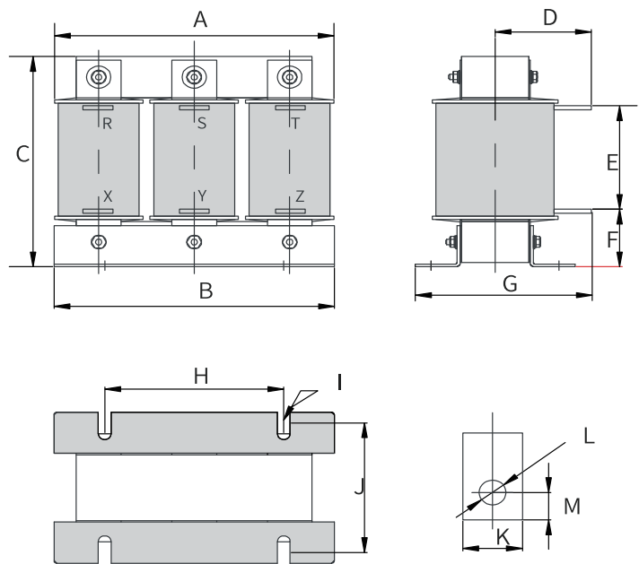
Figure 4-17 Dimensions of AC input reactors (80-120 A)
