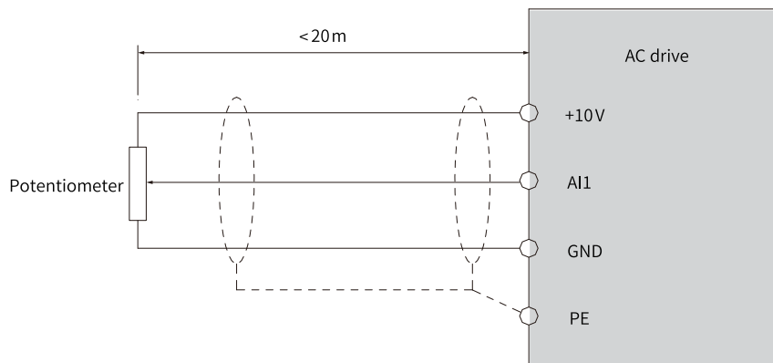
Figure 3-15 AI wiring
