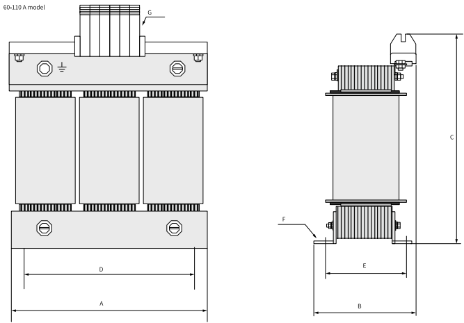
Figure 4-43 Dimensions of output reactors (60–110 A)
