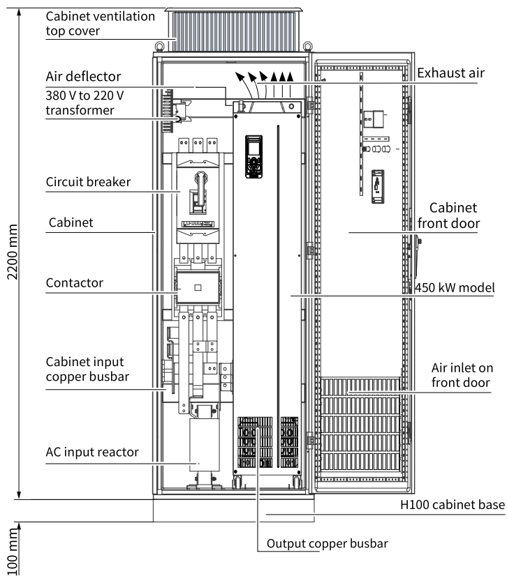
Figure 2-12 Recommended cabinet layout for T12 models
