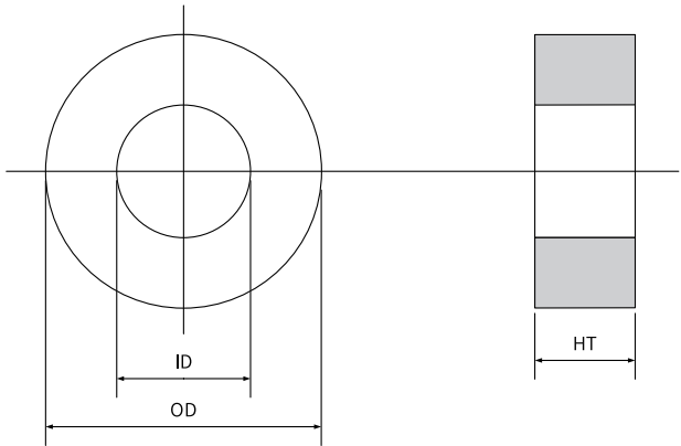
Figure 4-45 Dimensions of magnetic ring
