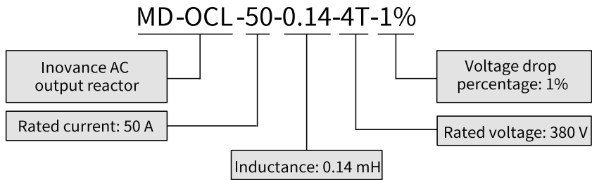
Figure 4-34 AC output reactor model
