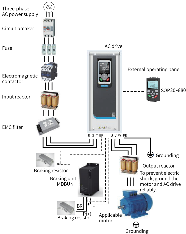
Figure 3-1 System structure
