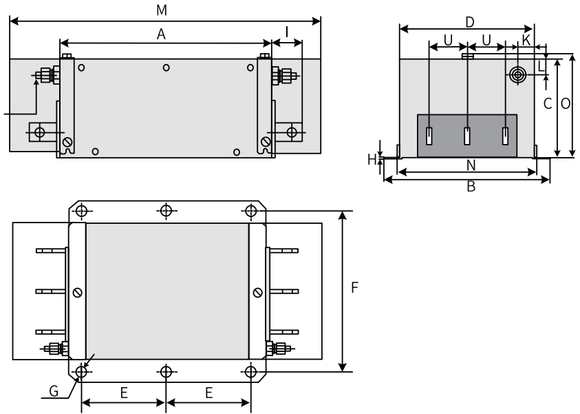
Figure 4-23 Dimensions of FN 3359 series filters (320-2500 A)
