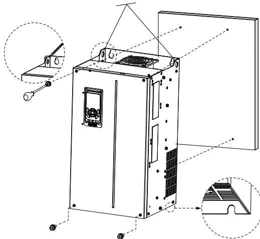
Figure 2-14 Backplate mounting (T7 to T9 models)
