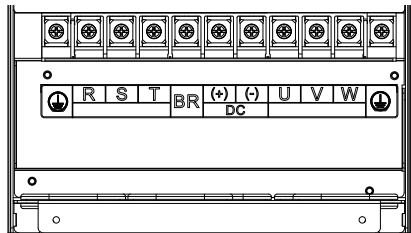
Figure 3-5 Layout of main circuit terminals for T5 to T8 models
