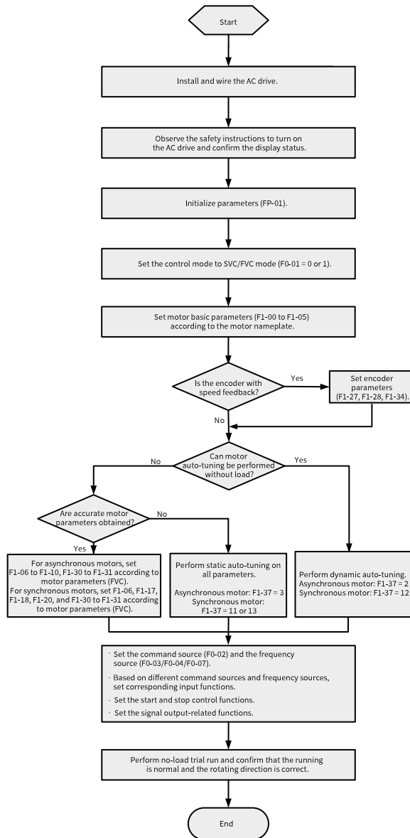
Figure 3-4 Commissioning process in SVC/FVC control mode
