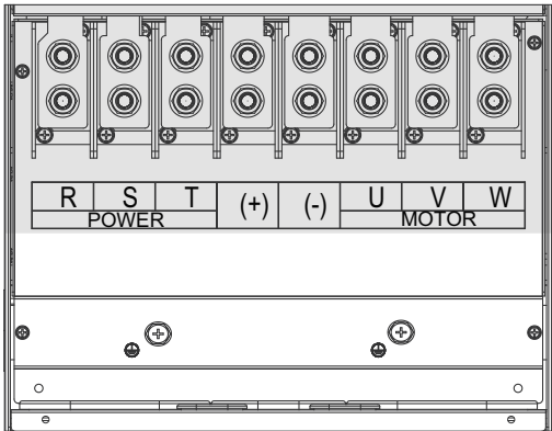
Figure 2-6 Main circuit terminals of T9 models
