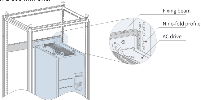
Figure 1-9 Perspective view of a cabinet for T11 and T12 models
