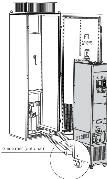
Figure 1-13 Aligning the casters with the guide rails
