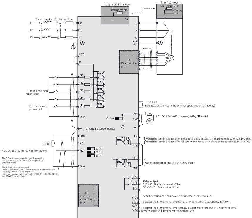
Figure 2-1 Standard wiring
