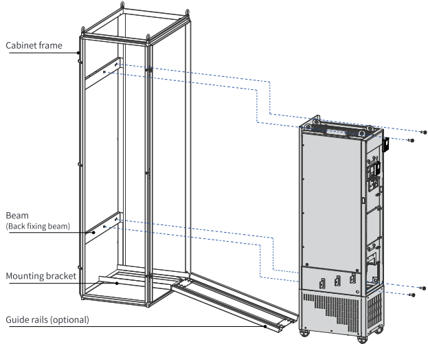
Figure 1-15 Fastening the AC drive to the fixing beams
