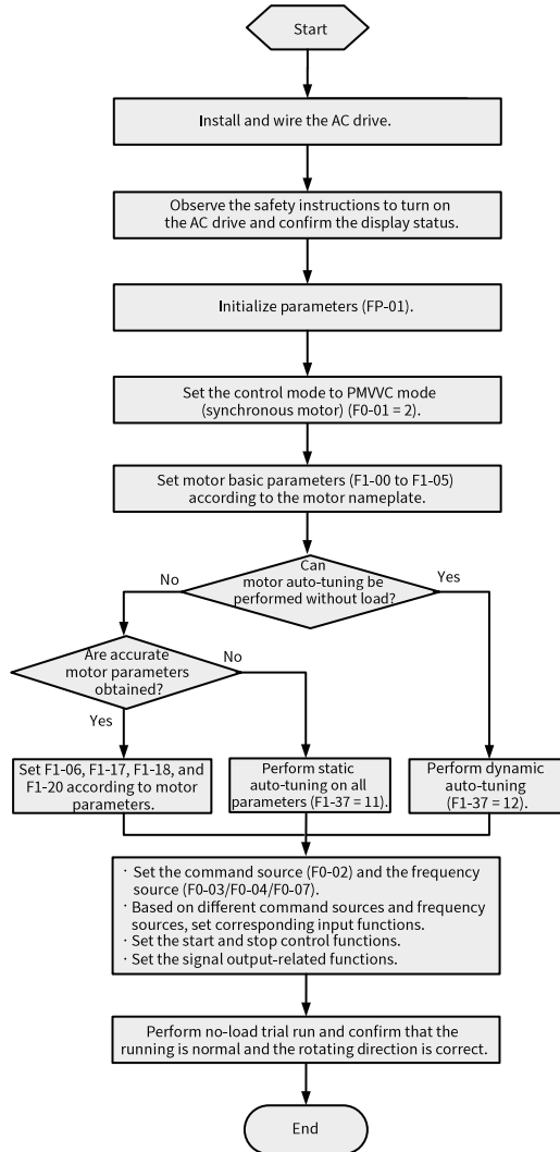
Figure 3-5 Commissioning process in PMVVC control mode
