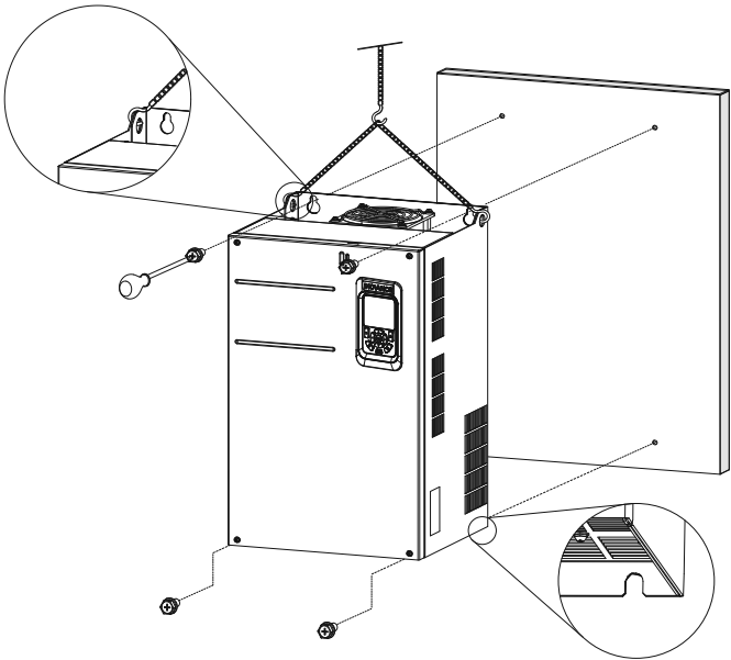
Figure 1-5 Backplate mounting (T7 to T9 models)
