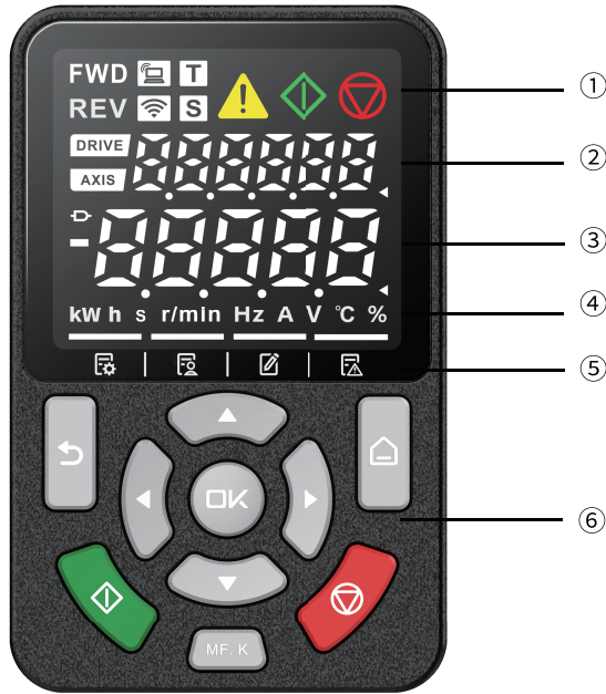
Figure 3-1 Operating panel display
