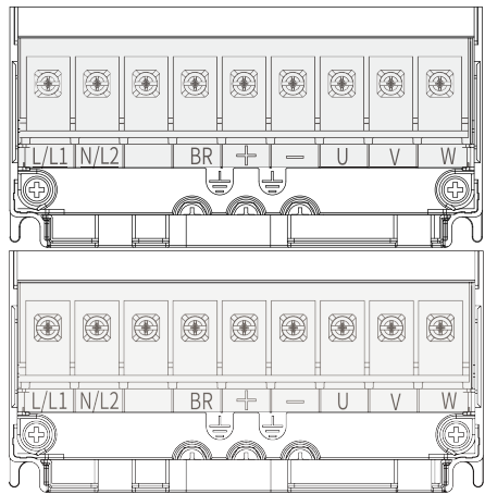
Figure 2-3 Main circuit terminals of T2 models (single phase)
