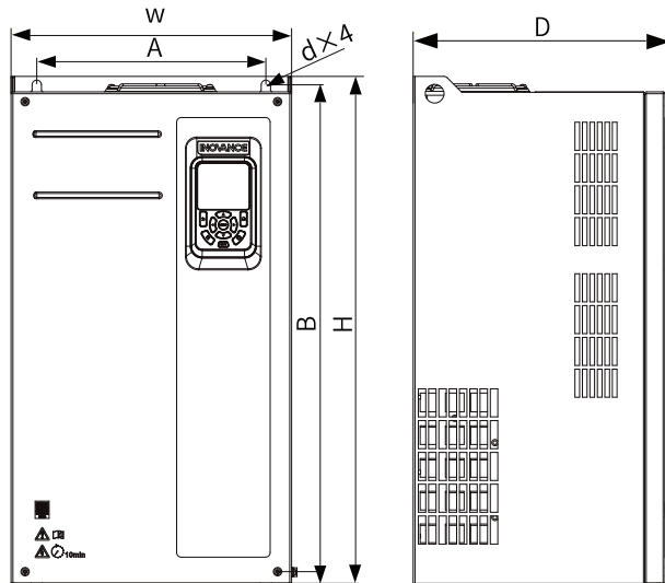
Figure 1-3 Outline dimensions and mounting dimensions of T7 to T9 models
