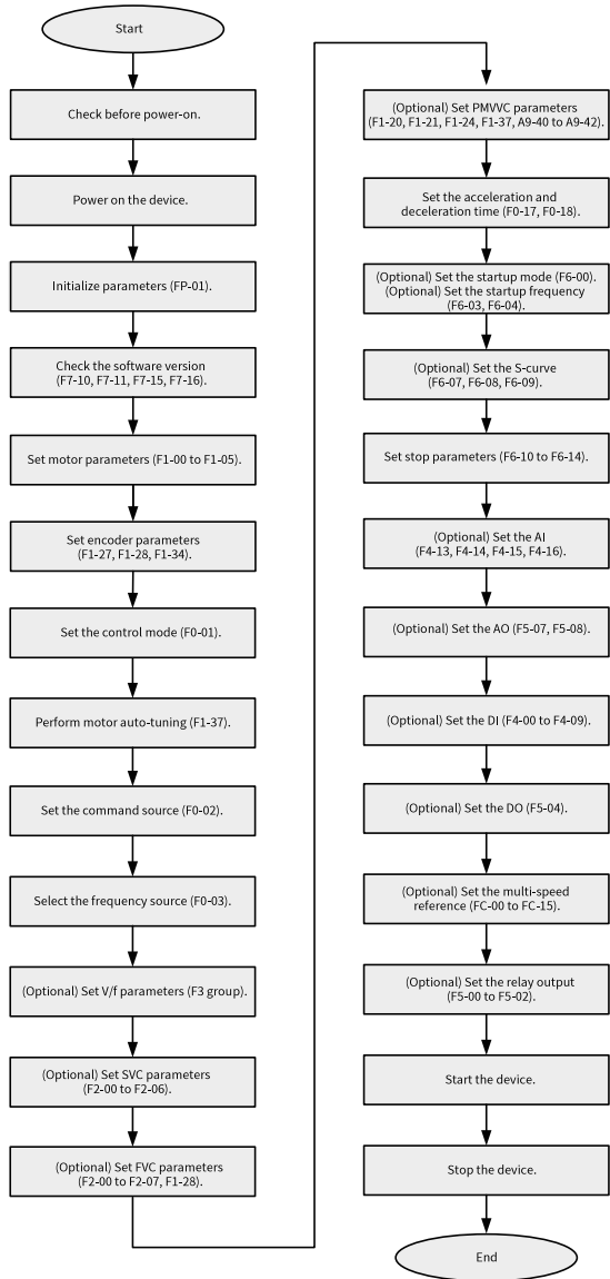
Figure 3-2 Commissioning process
