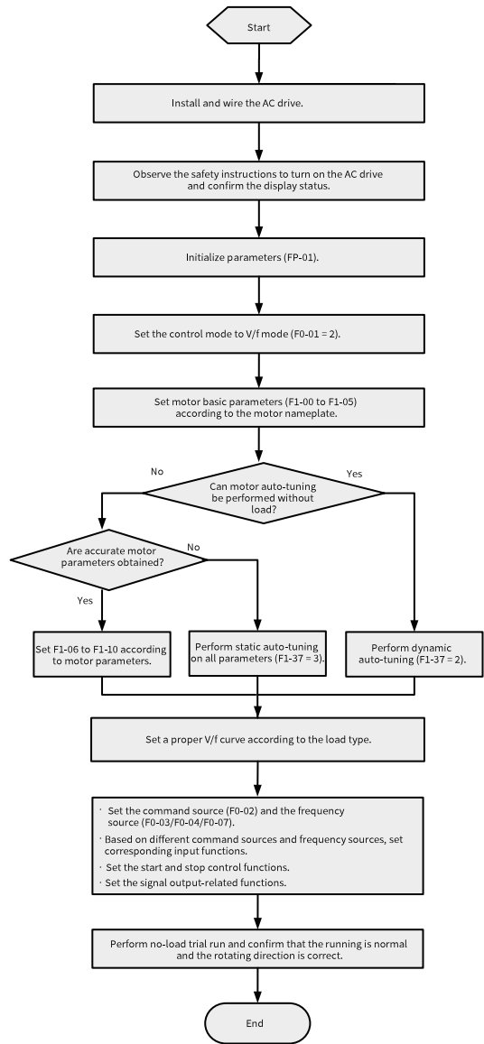
Figure 3-3 Commissioning process in V/f control mode
