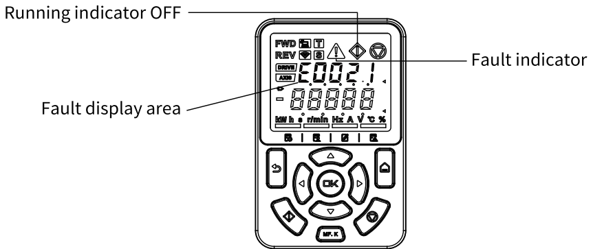
Figure 4-1 Display of faults
