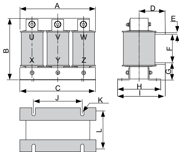
Figure 5-41 Dimensions of the AC output reactor (80-120 A)
