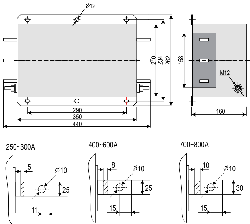
Figure 5-28 Dimensions of Jianli filters (250-800 A) (unit: mm)
