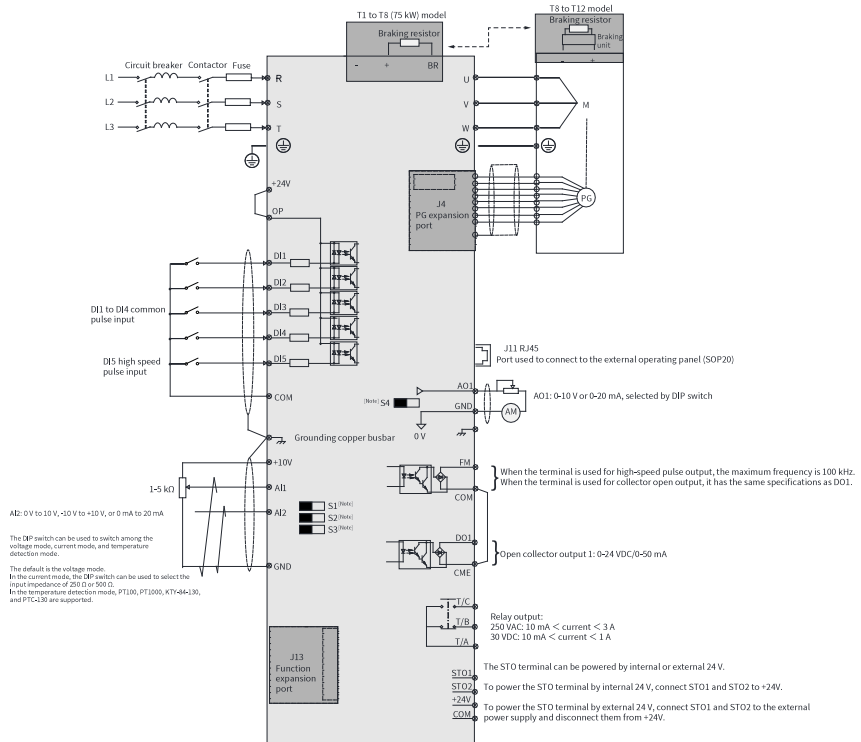
Figure 3-2 Standard wiring
