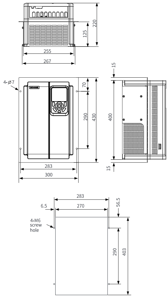
Figure 5-6 Dimensions of MD500-AZJ-A1T6 through-hole mounting bracket and holes (mm)
