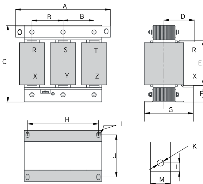
Figure 5-20 Dimensions of 150-330 A AC input reactors
