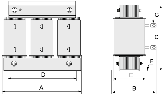
Figure 5-46 Dimensions of the output reactor (124–1100 A)
