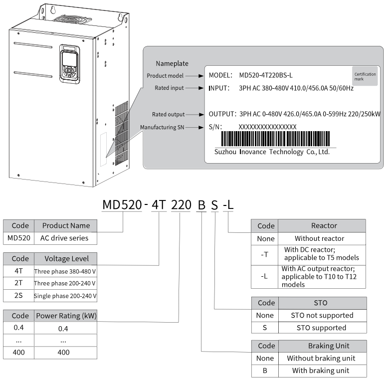
Figure 1-2 Nameplate and designation rule
