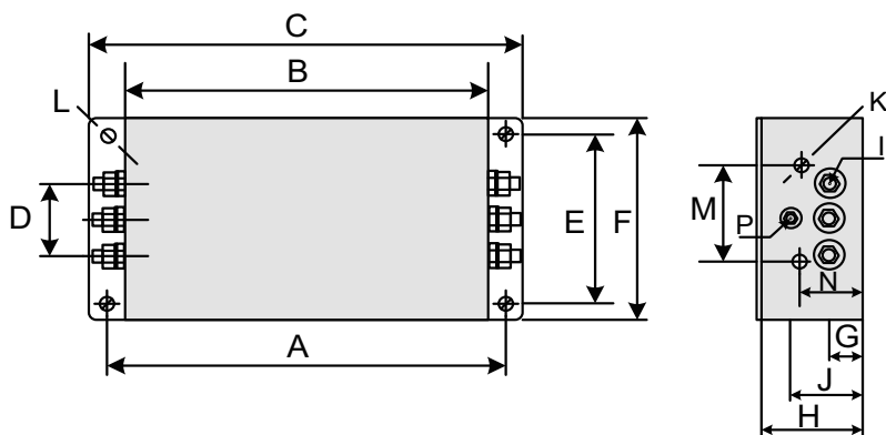
Figure 5-27 Dimensions of Jianli filters (50-200 A)
