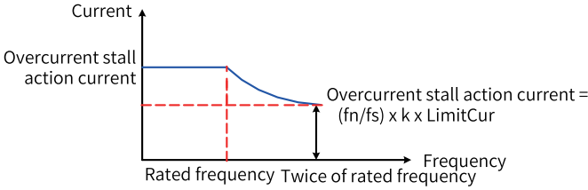
Figure 3-42 Speed multiplying overcurrent stall action current
