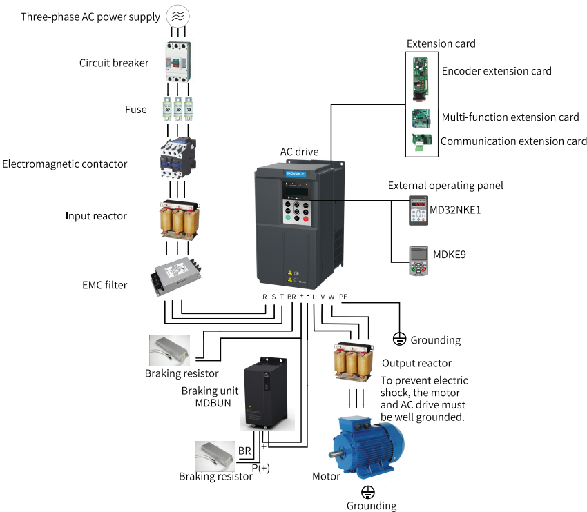
Figure 3-1 System structure
