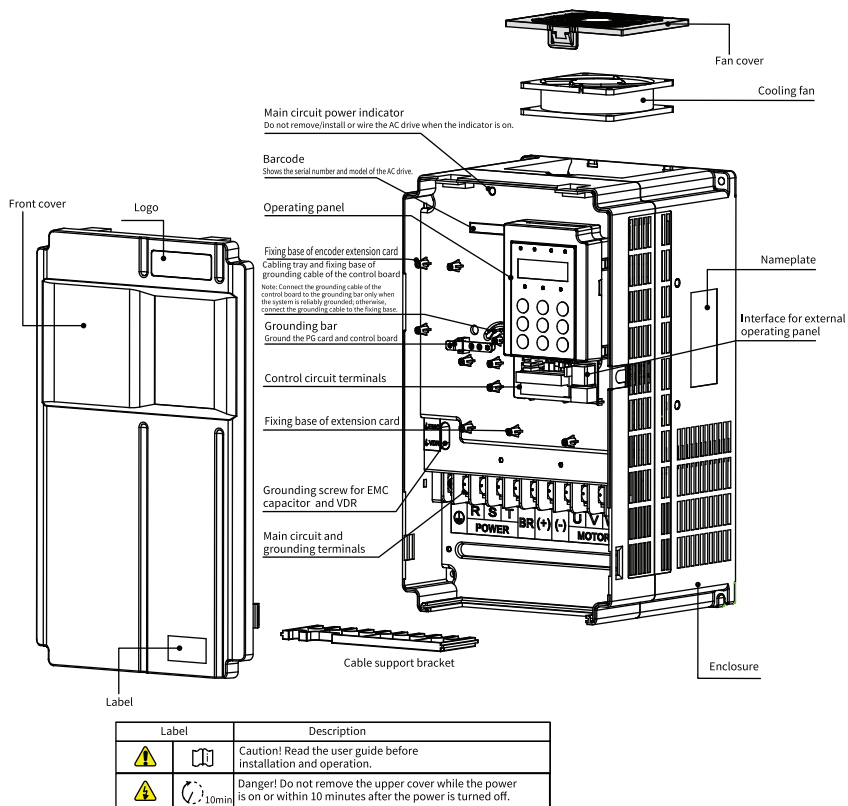
Figure 2-2 Components of T5 to T6 models
