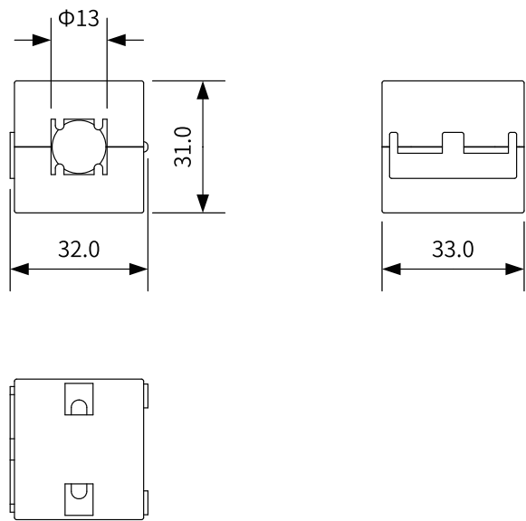
Figure 5-54 Dimension drawing of ferrite clamp
