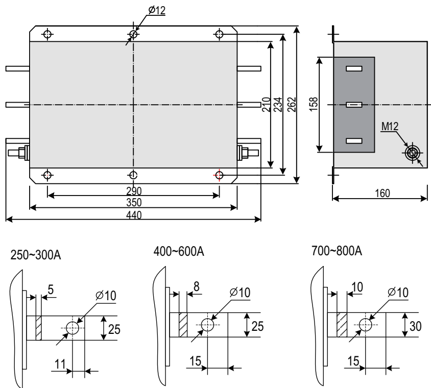
Figure 5-34 Dimension drawing of JIANLI filters (250 A to 800 A) (unit: mm)
