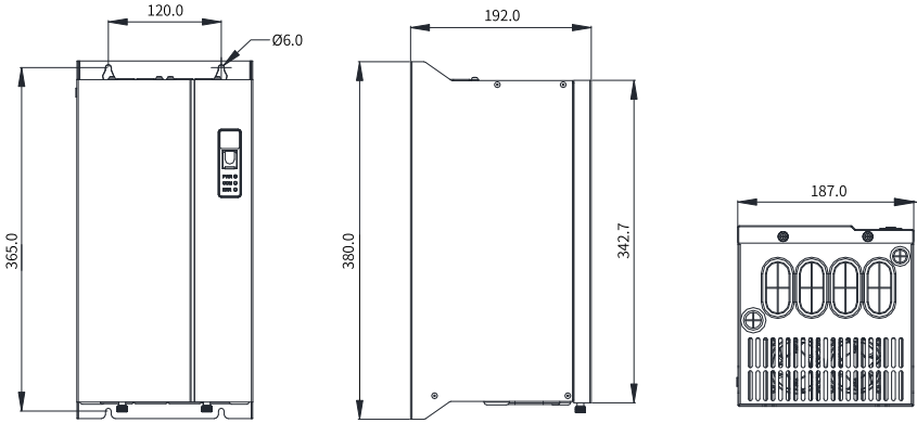
Figure 5-39 Dimensions of MDBUN series braking units (MDBUN-200-T, MDBUN-200-5T, and MDBUN-200-7T) (unit: mm)
