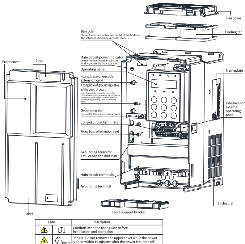
Figure 2-1 Components of T1 to T4 models
