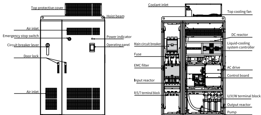
Figure 2-7 Components of standard cabinet with auxiliary power distribution cabinet
