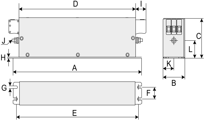
Figure 5-29 Dimension drawing of FN3258 series filters (50 A to 180 A)
