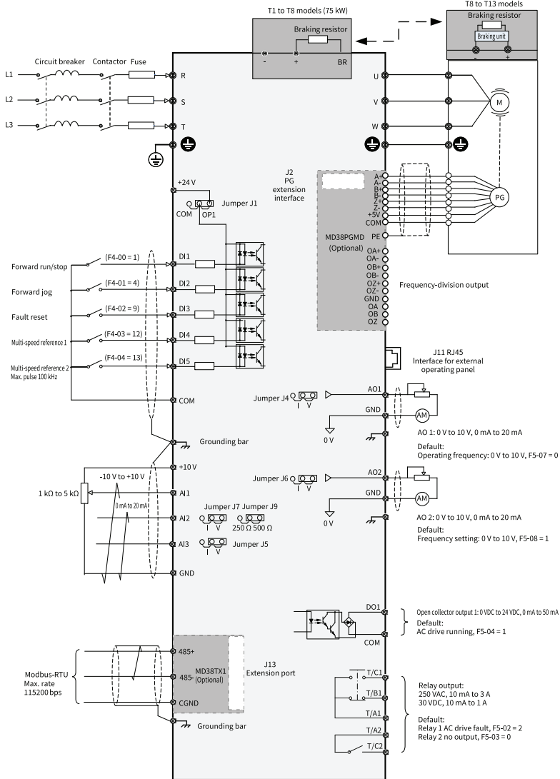
Figure 3-2 Standard wiring
