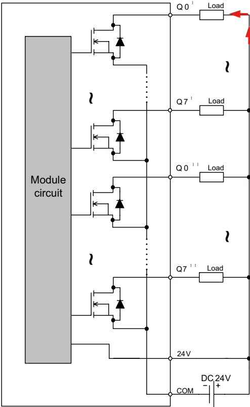
AM600-0016ETN output wiring diagram
