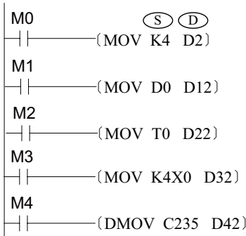
Ladder chart
