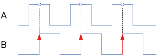
A phase leading B phase, counting up
