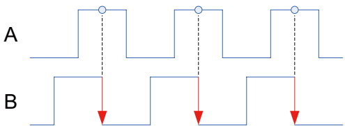
B phase leading A phase, counting down
