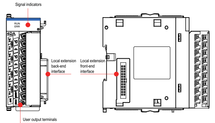
Figure 2 iagram of the analog output modules interface
