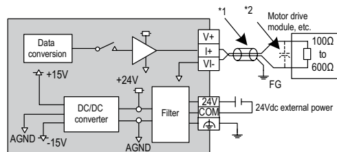
Figure 8 Connection for current-controlled signal
