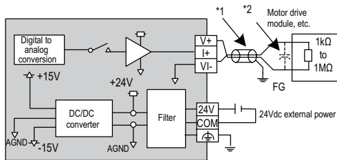
Figure 7 Connection for voltage-controlled signal
